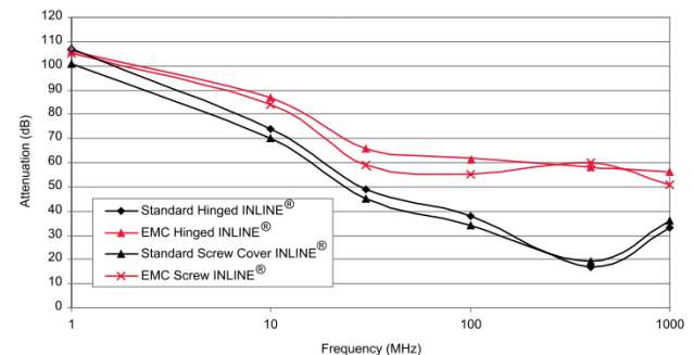
Figure 3. Hoffman INLINE ® Hinged Cabinet Shielding Effectiveness Standard Cabinet Compared to EMC Shielded Cabinet (see Appendix – Noise Mitigation Solutions).
