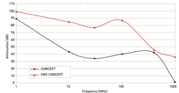
Figure 5. CONCEPT™ Shielding Effectiveness Standard Cabinet Compared to EMC Shielded Cabinet (see Appendix – Noise Mitigation Solutions).
