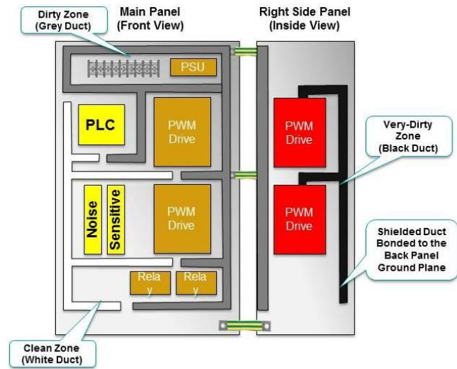
Figure 7. Typically, sources of EMI are placed on the right side of an enclosure, while victims of EMI are placed on the left side of an enclosure. To visually identify EMI sources and victims, black, white, and gray wiring duct is installed.
