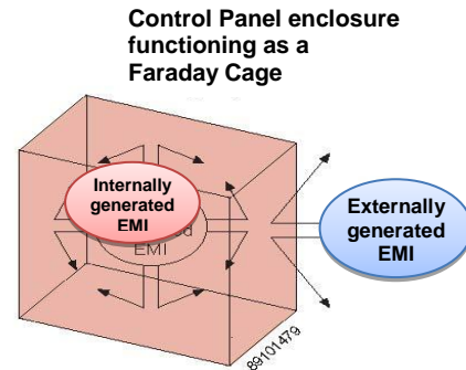
Figure 2. Effective enclosure design provides necessary user access while maximizing the Faraday cage effect when closed, controlling noise inside and outside of a control panel.
