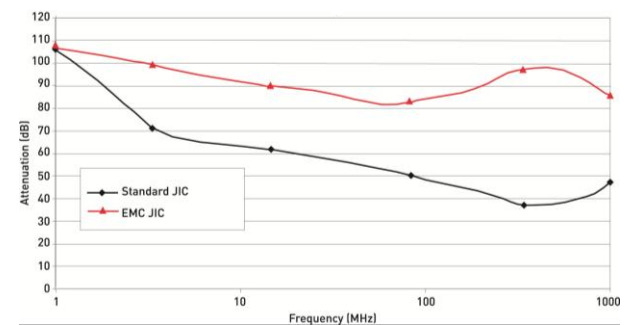
Figure 4. Steel JIC Shielding Effectiveness – Standard Mild Steel Compared to EMC Mild Steel JIC Cabinet (see Appendix – Noise Mitigation Solutions).
