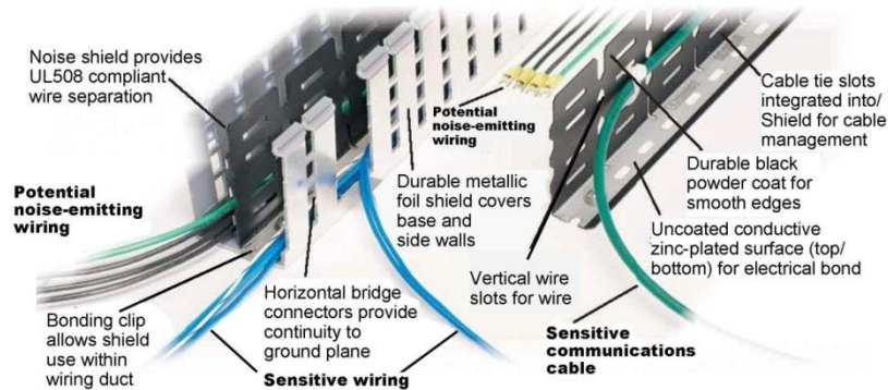
Figure 8. Noise shielding solutions can reduce the effects of EMI/RFI (electromagnetic interference, radio frequency interference) and provide space optimization within industrial control panels.
