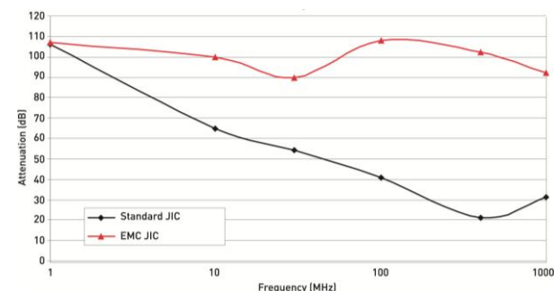
Figure 6. Stainless Steel JIC Shielding Effectiveness – Standard compared to EMC Stainless Steel JIC Cabinet (see Appendix – Noise Mitigation Solutions).
